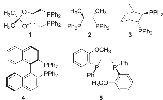
Scheme 1. Selected chiral diphosphane ligands for asymmetric catalysis.
