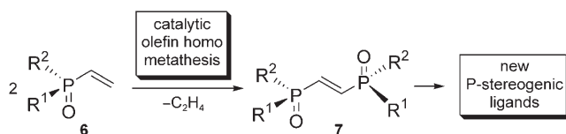
Scheme 2. Preparation of P-stereogenic 1,2-diphosphanylene dioxides 7 via homometathesis.
