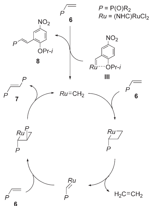
Scheme 6. Plausible mechanism for the formation of products 7 and 8 . NHC = 1,3-bis(2,4,6-trimethylphenyl)-2-imidazolidinylidene.
