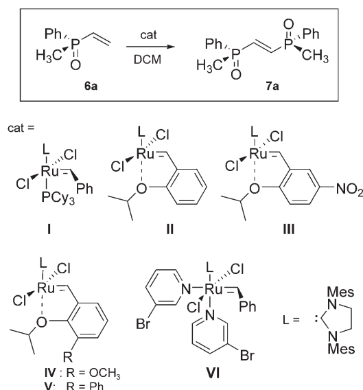
Scheme 3. Screening of the catalytic activity of complexes I–VI [54–58] in the homometathesis of ( S P )- 6a . Cy = cyclohexyl; Mes = 2,4,6-trimethylphenyl.
