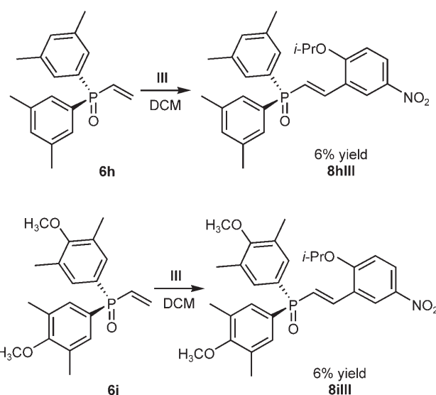
Scheme 5. Reagents and conditions: [a] 10 mol % of precatalyst III , DCM, 24 h, reflux. Isolated yields of analytically pure products.
