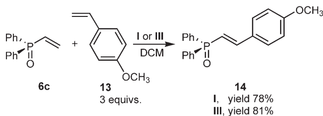
Scheme 7. Cross metathesis of 6b with electron-rich Type I styrene 13 .
